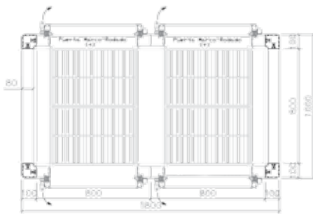
AMD/P 1803 [Puertas a ambas caras] 1000x1800x80 Ht: 2120 [+]
